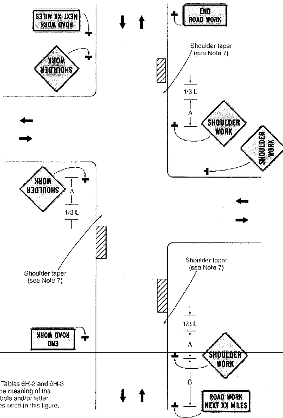
Typical Application 3
